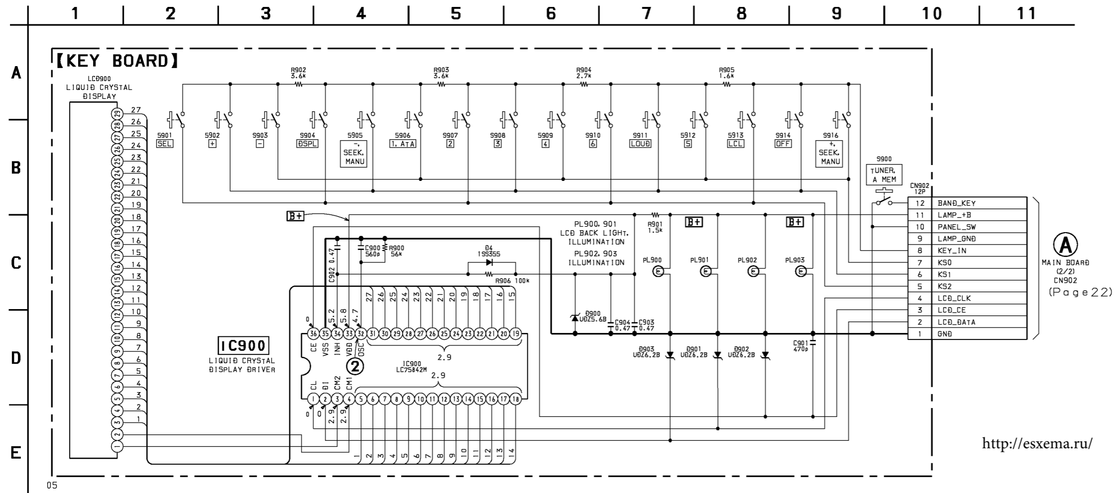
5-7. SCHEMATIC DIAGRAM – PANEL Section –
